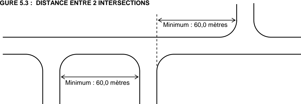
FIGURE 5.3 : DISTANCE ENTRE 2 INTERSECTIONS
